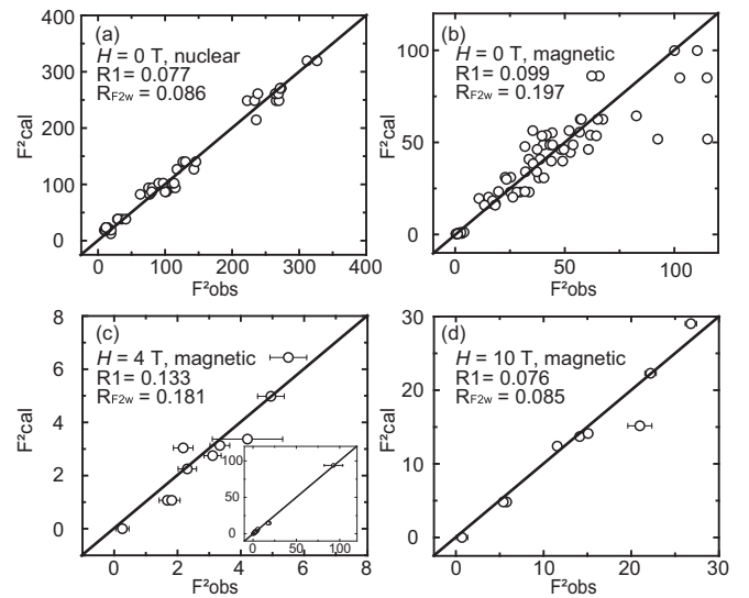
FIG. 8. Comparison of the squared magnetic structure factors between observations and calculations. (a) Nuclear peaks measured at zero field. (b) Magnetic peaks measured at zero field. (c) Magnetic peaks measured at H = 4 T. The inset shows stronger magnetic peaks at the wave vector \mathbf{k} = (0, 0, 1) . (d) Magnetic peaks measured at H = 10 T. The agreement factor is indicated on each panel.
