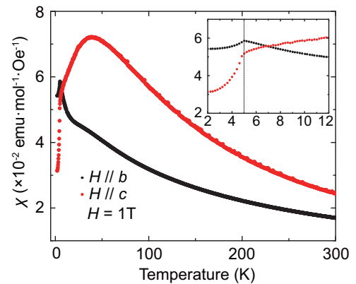
FIG. 2. Magnetic susceptibility measurements on \text{SrCo}_2\text{V}_2\text{O}_8 single crystal under magnetic field H = 1 T applied along the b and c directions. The inset shows the magnetic susceptibility curves near the transition temperature. The vertical line at 5 K indicates the transition temperature.
