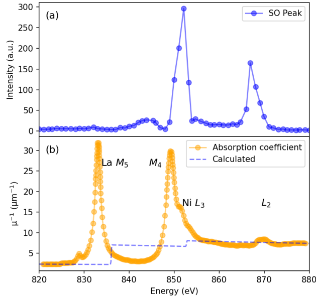
FIG. S1 (a) Experimental intensities of the (0.36, 0.36, 0) spin-order superstructure peak as a function of photon energy at 70K for \pi -polarized x-rays. \pi -polarized x-rays were used to enhance the magnetic signal from the sample and reduce background. (b) Estimated x-ray absorption coefficient for the LSNO sample. This was completed by scaling the pre-edge and post-edge regions of the x-ray absorption coefficient with the calculated one as labeled by blue dashed line in (b) [1]. The corresponding x-ray absorption spectrum is extracted from Ref. [2] for a similar sample to ours. We can estimate from (b) that the estimated penetration depth is \sim 69 nm when the energy of the incident x-ray is 852 eV and the incidence angle \alpha_i of the x-ray is 75.4^\circ .
