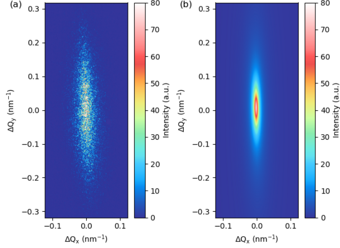
FIG. S2 (a) Representative coherent x-ray diffraction patterns from the SO superlattice peaks at \mathbf{Q} = (0.36, 0.36, 0) , which is measured with an 8\ \mu\text{m} pinhole. Here, \Delta\mathbf{Q} = \mathbf{q} - \mathbf{Q} and \mathbf{q} is the scattering wavevector transfer. (b) Result of a 2D fit of (a) to a Lorentzian squared function.
