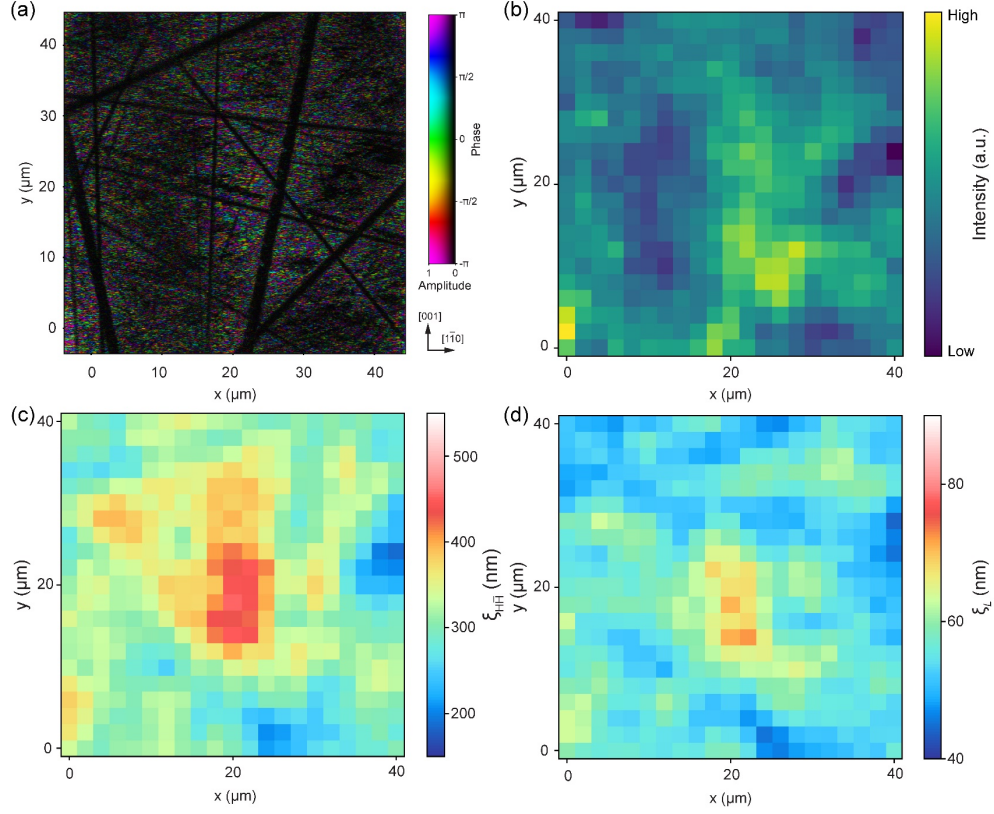
FIG. S4 (a) Representative ptychographic image of SO stripe domains over a large scale. The image has been aligned to the crystal orientation of the LSNO sample as shown in the legend of the figure. Here, the amplitude is represented by the brightness of the image and the phase is rendered by the hue. (b) Integrated coherent x-ray diffraction intensity. (c) SO domain size along [1\bar{1}0] . (d) SO domain size along [001] directions. The most striking features in (a) are the straight dark lines which resemble the scratches due to crystal polishing. It is possible the scratches are filled by (1\bar{1}0) SO stripe domains, but we suspect the disappearance of the SO domains in these regions may result from the surface damage of the sample due to polishing.
