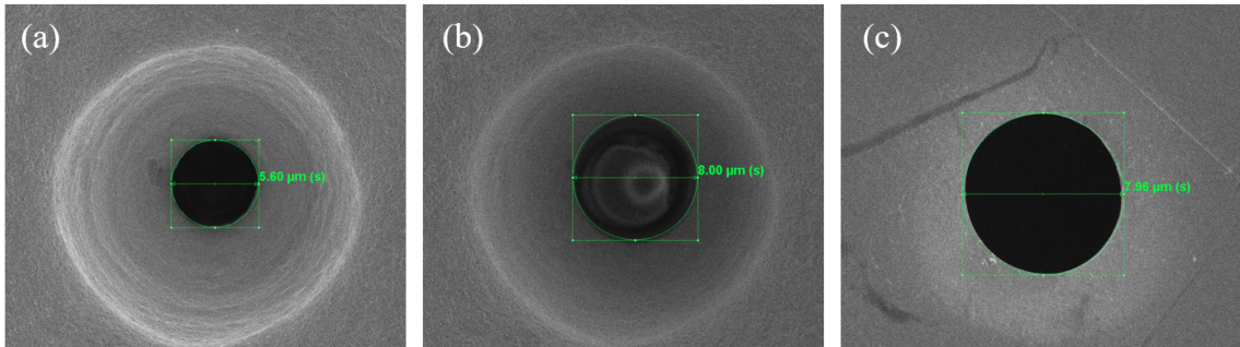
FIG. S3 Scanning electron microscope images of the pinhole before and after Focused Ion Beam (FIB) polish. (a) Back view of the pinhole before FIB polish. (b) Back view of the pinhole after FIB polishing. (c) Front view of the pinhole after FIB polishing.
