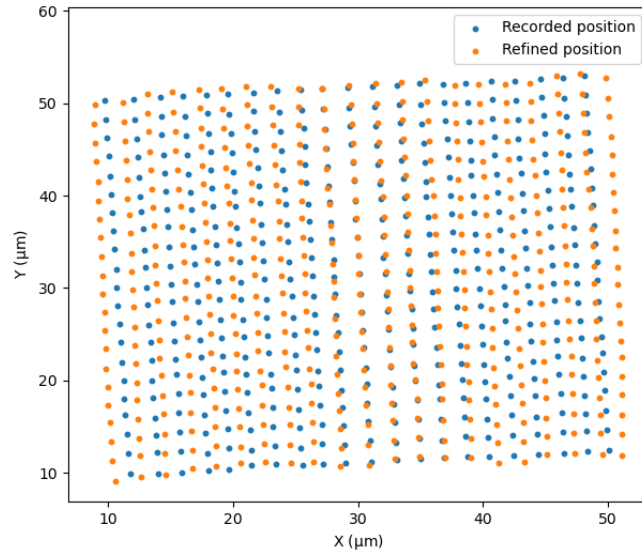
FIG. S6 Plot of the refined positions for the reconstruction of LSNO data. Here, the blue dots represent the recorded x-ray probe positions in the detector frame on the LSNO sample during the ptychography experiment. The orange dots show the refined x-ray probe position in detector frame by using the annealing method.
