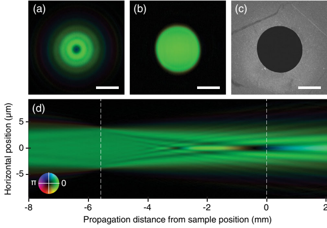
FIG. 2. (a) Reconstructed complex-valued wavefront of x-ray probe along the incident x-ray direction at the LSNO sample position. Here, the amplitude is mapped by the image brightness, and the corresponding phase is mapped by hue. (b) Computed free space propagation of the reconstructed soft x-ray probe to the plane where the pinhole was placed. (c) SEM image of the 8 \mu\text{m} pinhole. (d) Horizontal cut through the propagated wavefield, displaying the waist of the soft x-ray beam in the pinhole plane. Here, the left dashed lines show the position of the pinhole and the right dashed line shows the LSNO sample position. Scale bars are 4 \mu\text{m} .
