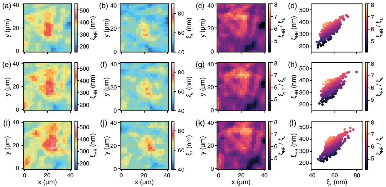
FIG. 5. (a),(e),(i) SO domain sizes extracted directly from the diffraction patterns along [110] . (b),(f),(j) Same along [001] . (c),(g),(k) The ratio between the two directions as a function of the scanning position. (d),(h),(l) The corresponding ratio distribution. (a)–(d), (e)–(h), and (i)–(l) were at 0, 31, and 94 min, respectively.
