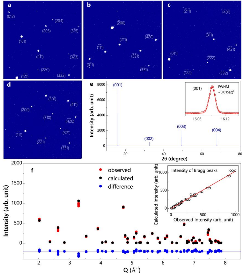
Supplementary Figure 2: Single crystal X-ray diffraction data and the Rietveld refinement results in FeSe.
