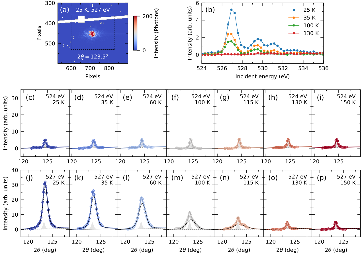
FIG. S1. Fitting of the REXS data at O K -edge. (a) A representative detector image of the superlattice peak at Q=(0.5, 0, 0) . The dashed lines envelop the region of interest in which the pixel readings are summed up to extract the peak intensity. The white pixels originate from the beamstop/detector errors that have been removed from the data. (b) Incident energy dependence of the superlattice peak intensity at different temperatures. The small energy shift ( < 0.3 eV) between the energy scans of different temperature is due to the photon energy change associated with the monochromator that is sensitive to thermal perturbations. (c)-(p) A series of theta-2theta scans with different incident energy and temperature. The circles are the data and the solid lines are the fitting results which can be further broken into several components including a sloped background (gray dashed lines), a pseudo-Voigt function presenting the second harmonic of the Bragg peak (gray shaded area) and another pseudo-Voigt function outlining the magnetic contributions (black dashed lines).
