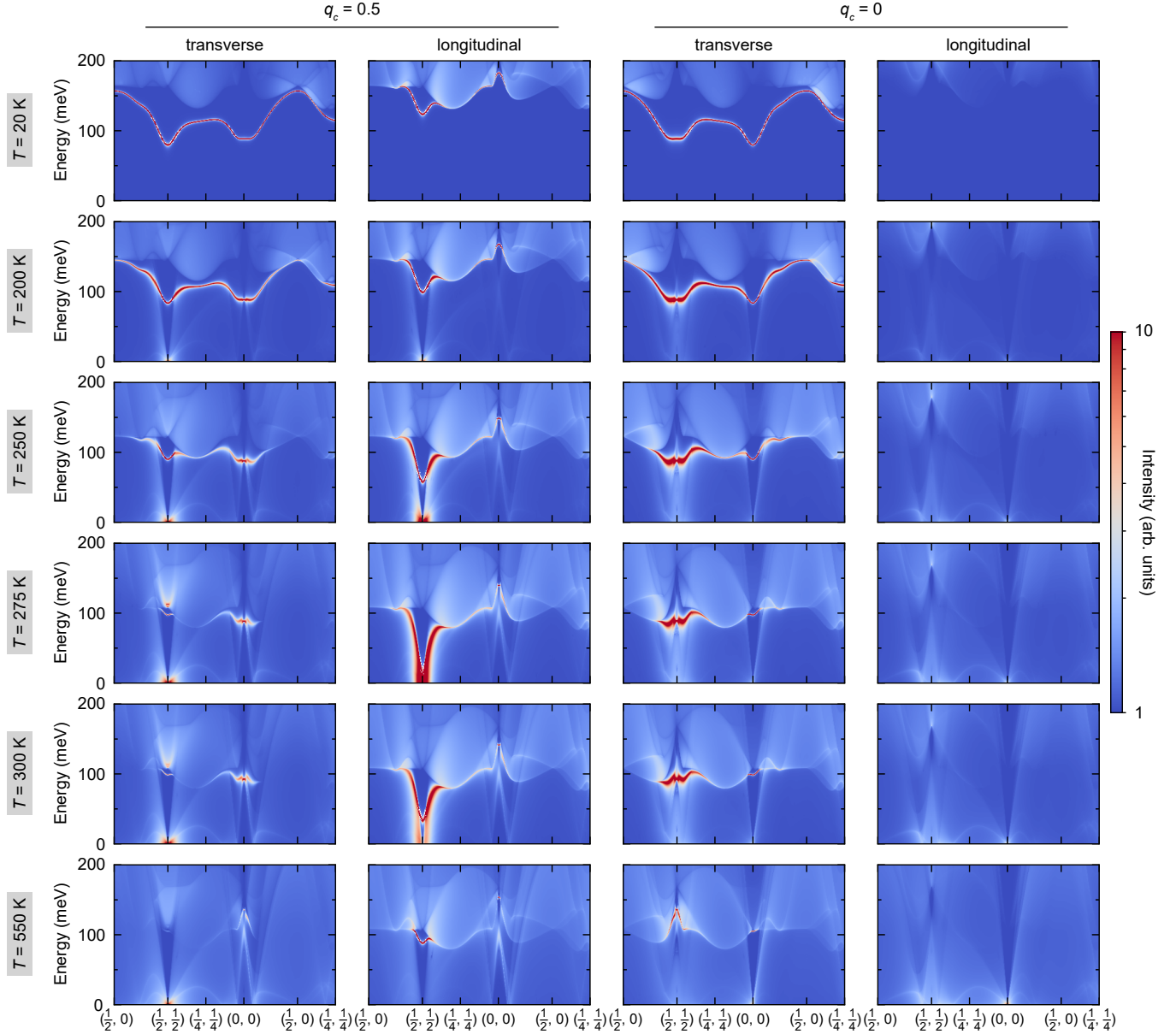
FIG. S5. Theoretical prediction of excitonic mode condensation at T_N . Theoretical calculation of the transverse and longitudinal magnetic excitation spectrum at q_c = 0 and 0.5 as function of temperature. The color bar indicates the strength of the magnetic excitations.
