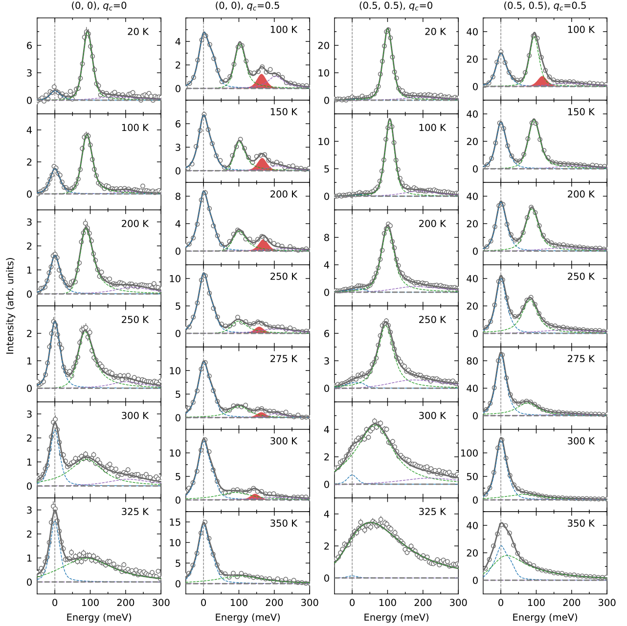
FIG. S2. Temperature dependence of energy-loss spectra at (0, 0) and (0.5, 0.5). RIXS spectra at (0, 0) and (0.5, 0.5) with q_c = 0 and 0.5 for specific temperatures. The black circles represent the data and dotted lines outline the different components of the spectrum, which are summed to produce the solid line representing the total spectrum. The fitting procedure is described in detail in the Methods section of the main manuscript. Error bars are determined using Poissonian statistics. The results support the longitudinal mode condensation at T_N .
