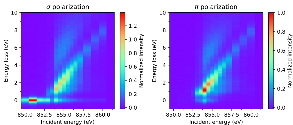
Fig. 2 Ni L_3 -edge RIXS energy map for \text{La}_4\text{Ni}_3\text{O}_{10} measured at 25 K with an incident angle of \theta_i = 15^\circ and scattering angle of 2\Theta = 95^\circ . The left and right panels show \sigma and \pi incident x-ray polarization, respectively.
