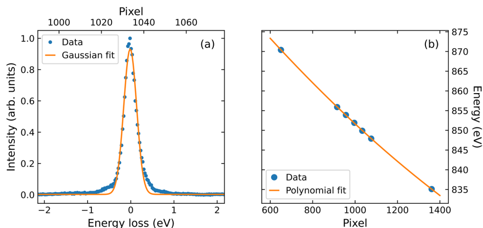
Fig. 6 RIXS instrument parameters. (a) Elastic line measurement; a gaussian fit yields \text{FWHM} = 262 \pm 9 meV. (b) Dispersion of the elastic line through the CCD detector, the calibration follows a second order polynomial ( y = a + bx + cx^2 ) with a = 912.7 eV, b = -7.24 \times 10^{-2} eV/pixel, and c = 1.13 \times 10^{-5} eV/pixel 2 .
