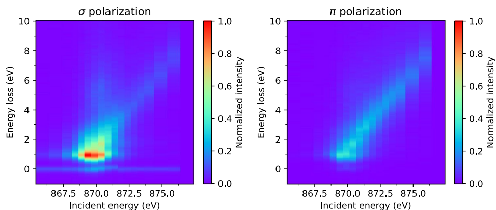
Fig. 4 Ni L_2 -edge RIXS energy map for \text{La}_4\text{Ni}_3\text{O}_8 measured at 25 K with an incident angle of \theta_i = 15^\circ and scattering angle of 2\Theta = 95^\circ . The left and right panels show \sigma and \pi incident x-ray polarization, respectively.
