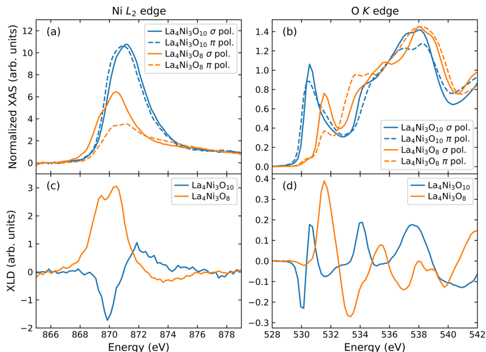
Fig. 5 XAS measurements of \text{La}_4\text{Ni}_3\text{O}_{10} and \text{La}_4\text{Ni}_3\text{O}_8 taken at 300 K and \theta_i = 15^\circ . The Ni L_2 edge XAS and XLD are displayed in panels (a,c), respectively. Panels (b,d) display the O K edge XAS and XLD, respectively.
