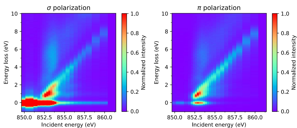
Fig. 3 Ni L_3 -edge RIXS energy map for \text{La}_4\text{Ni}_3\text{O}_8 measured at 25 K with an incident angle of \theta_i = 15^\circ and scattering angle of 2\Theta = 95^\circ . The left and right panels show \sigma and \pi incident x-ray polarization, respectively.
