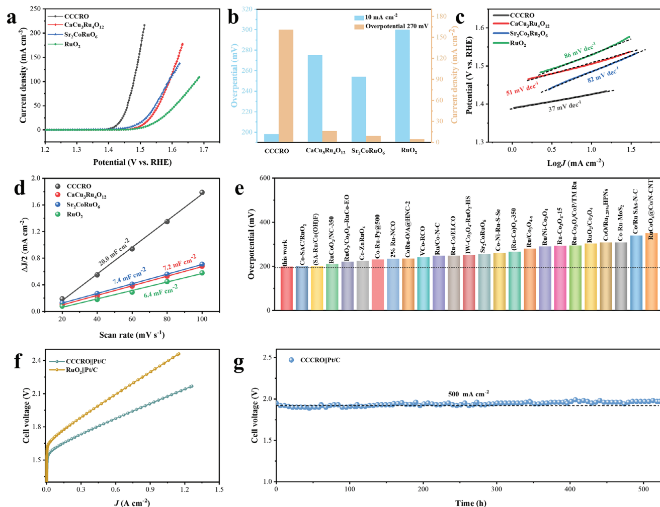
Figure 3. Electrocatalytic OER performance. a) LSV curves of CCCRO, \text{CaCu}_3\text{Ru}_4\text{O}_{12} , \text{Sr}_2\text{CoRuO}_6 , and \text{RuO}_2 . b) Comparison of the overpotentials (at current density of 10 \text{ mA cm}^{-2} ) and the current densities (at an overpotential of 270 \text{ mV} ) of the CCCRO, \text{CaCu}_3\text{Ru}_4\text{O}_{12} , \text{Sr}_2\text{CoRuO}_6 , and \text{RuO}_2 . c) Tafel plots. d) Differences in the charging current density plotted against the scan rate for CCCRO, \text{CaCu}_3\text{Ru}_4\text{O}_{12} , \text{Sr}_2\text{CoRuO}_6 , and \text{RuO}_2 . e) Comparison of the overpotential at 10 \text{ mA cm}^{-2} for CCCRO and the previously reported Co-Ru based catalysts. f) LSV curves of the AEM electrolyzer using CCCRO and \text{RuO}_2 , Pt/C catalysts as the anodic and cathodic electrodes, respectively. g) Stability tests of the AEM water electrolyzers at 500 \text{ mA cm}^{-2} .
