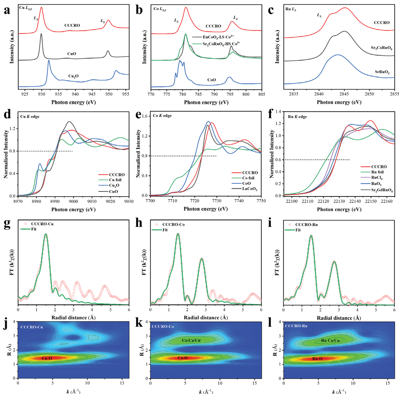
Figure 2. Characterization of valence and coordination structures. a) Cu L_{2,3} -edge spectra of CCCRO (red line) and references Cu 2+ O (black line) and Cu + 2 O (blue line). b) Co L_{2,3} -edge spectra of CCCRO (red line) and references LS-Co 3+ (EuCo 3+ O 3 : black line), HS-Co 3+ (Sr 2 Co 3+ RuO 6 : green line), and Co 2+ O (blue line). c) Ru L_3 -edge spectra of CCCRO (red line) and references Sr 2 CoRu 5+ O 6 (black line) and SrRu 4+ O 3 (blue line). d) Cu K-edge spectra of CCCRO (red line) and references Cu 0 foil (green line), Cu 2+ O (black line), and Cu + 2 O (blue line). e) Co K-edge spectra of CCCRO (red line) and references Co 0 foil (green line), LaCo 3+ O 3 (black line), and Co 2+ O (blue line). f) Ru K-edge spectra of CCCRO (red line) and references Sr 2 GdRu 5+ O 6 (black line), Ru 4+ O 2 (blue line), Ru 3+ Cl 3 (purple line), and Ru 0 foil (green line). g–i) The EXAFS fitting curves for CCCRO. j–l) WT for the k^2 -weighted EXAFS spectra of CCCRO.
