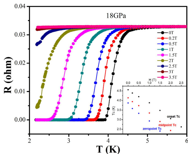
Figure 3. The superconducting transitions of HfTe 5 with applied magnetic field H perpendicular to the ac plane of HfTe 5 single crystal at 18 GPa. The inset shows T c evolution as function of magnetic field H.
