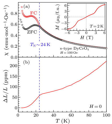
Fig. 3. Magnetic and thermal-expansion properties of the s-type \text{DyCrO}_4 . (a) Temperature dependence of ZFC and FC magnetic susceptibility measured at 100 Oe. The inset shows the isothermal magnetization measured at 2 K. (b) Temperature dependence of linear thermal expansion. The dashed line indicates the antiferromagnetic (AFM) phase transition and thermal expansion anomaly at T_N .
